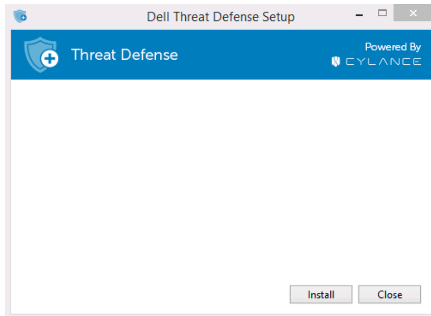
Figure 29: Setup Window
