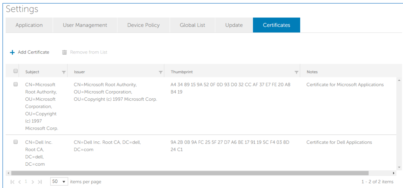
Figure 25: Certificate Repository
